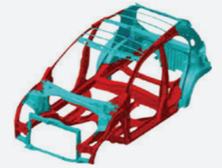
GCON Body Structure
