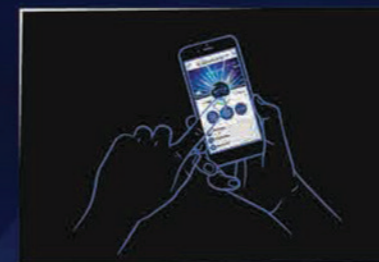
Vehicle Dashboard
