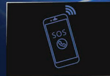
Emergency Call
