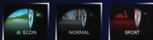
Drive Mode *
